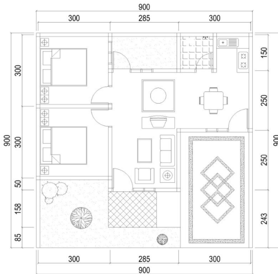
DENAH TYPE 45
